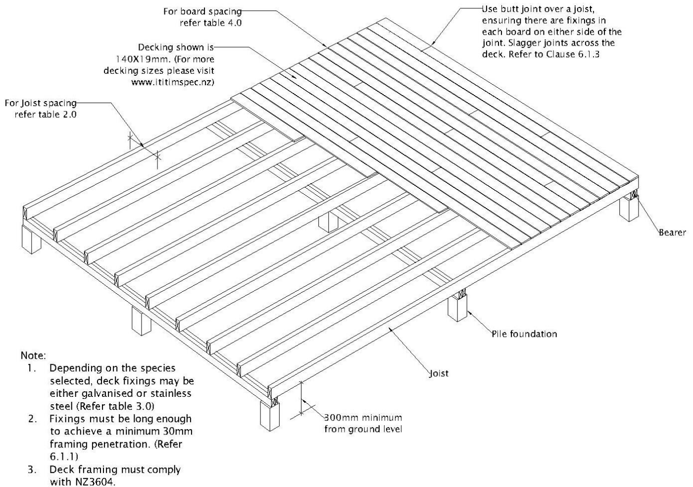
Figure 1 Decking Installation Drawing
